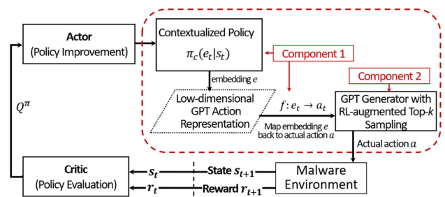
Fig. 4. The abstract view of AC-CAR Architecture. Component 1 includes the actor network operating in a low-dimensional action representation obtained from GPT’s embedding space. This embedding is subsequently mapped to the environment’s actions using function f . Component 2 leverages these actions as initial context to generate evasive contents using a modified top- k sampling procedure.
